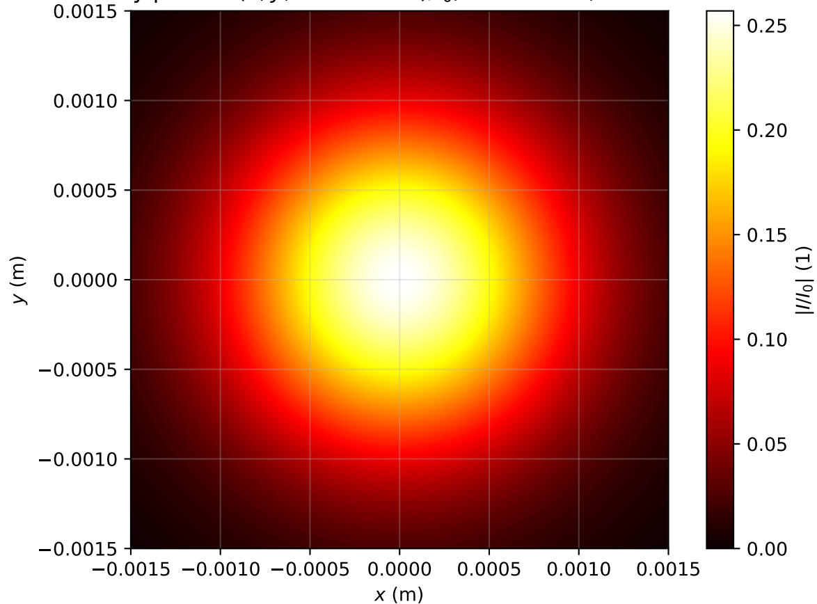
Intensity profile I(x, y, z = 3.901m)/I_0 , P_{in}=0.2P_{cr} , artificial time
